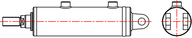
STYLE FC FEMALE CLEVIS
