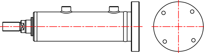
STYLE RF REAR FLANGE
