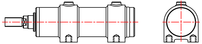
STYLE TM SPHERICAL BRG
