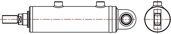
STYLE MCSB SPHERICAL BRG
