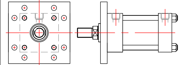
STYLE 4 NFPA MF5 HEAD SQUARE FLANGE
